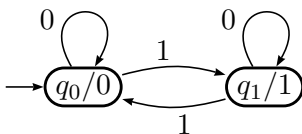
FIGURE 1. The finite-state automaton recognizing the set of Thue–Morse integers.
